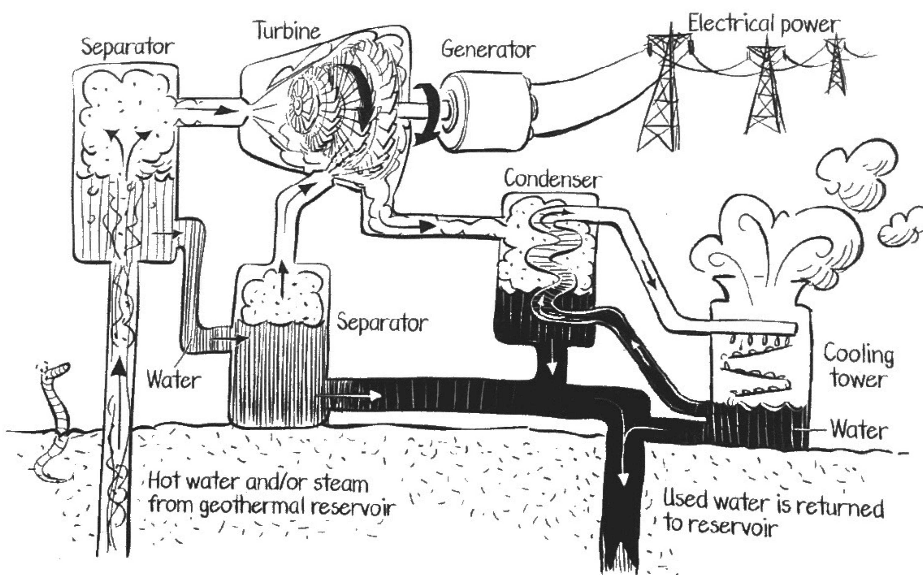
Flash steam plants can include one steam/water separator or, more commonly, two separators (shown here).
