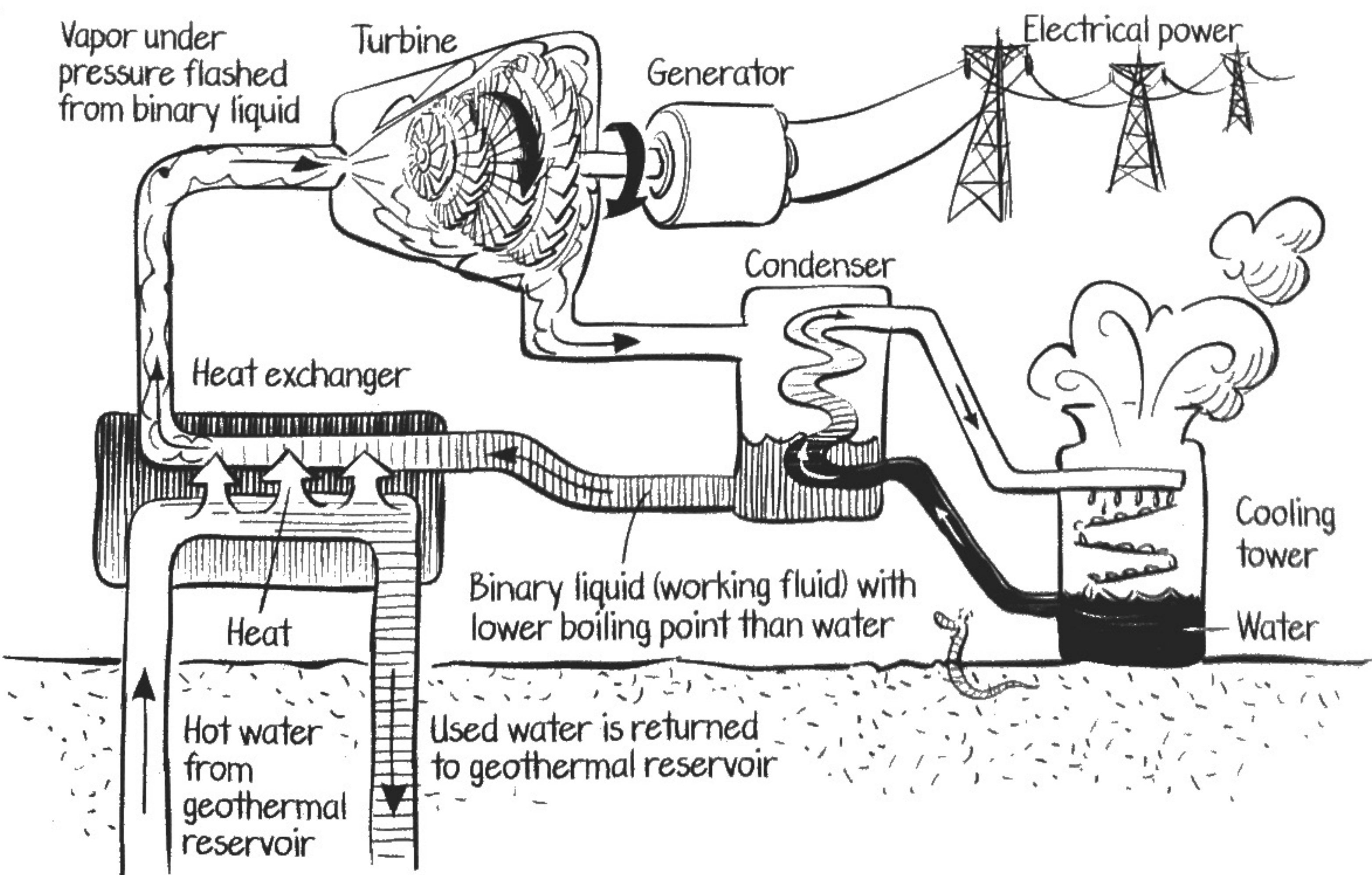
Binary power plant
